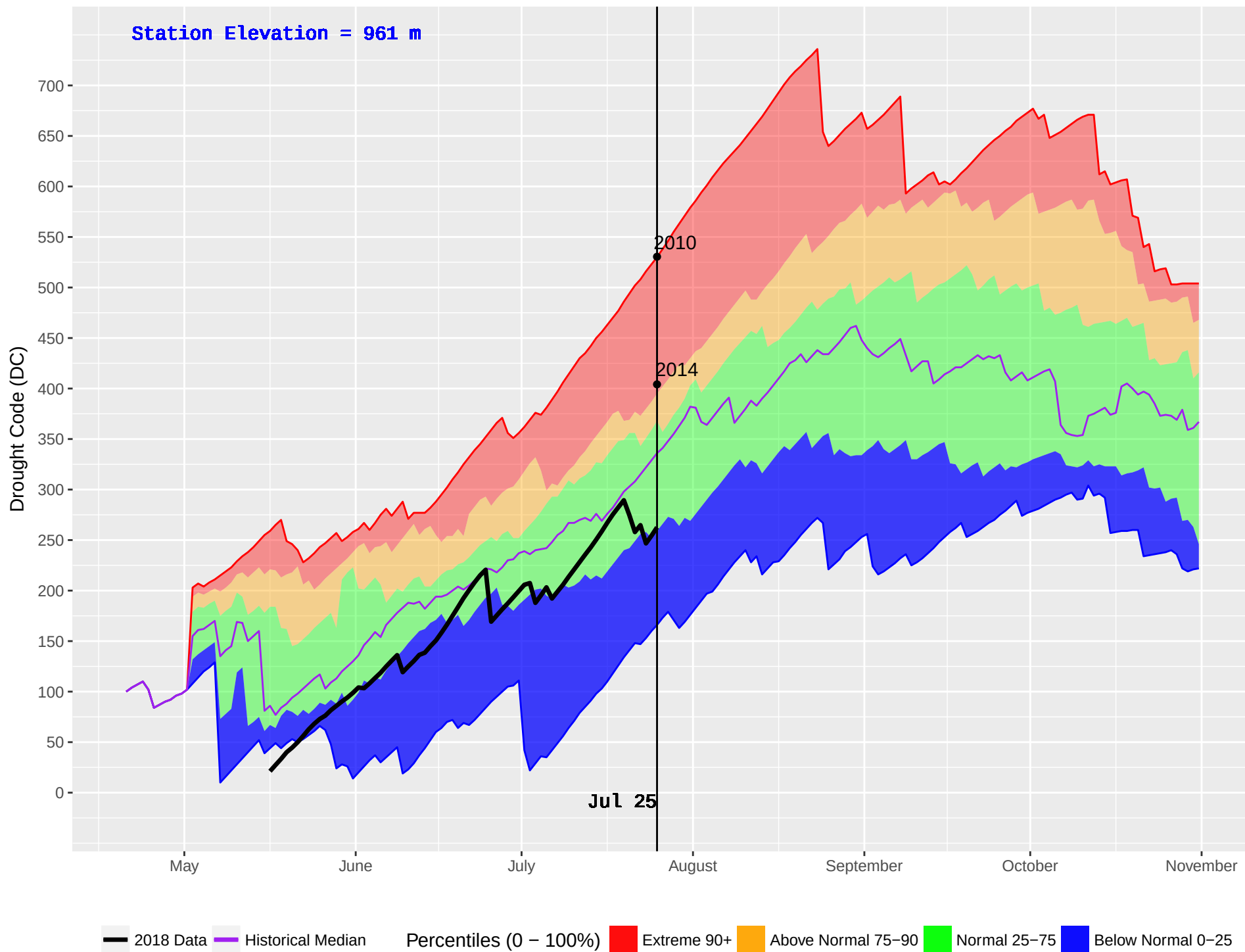
HOLY CROSS 2 (654) : Historical (1998–2016) and Current (2018) Noon Drought Code (DC)
