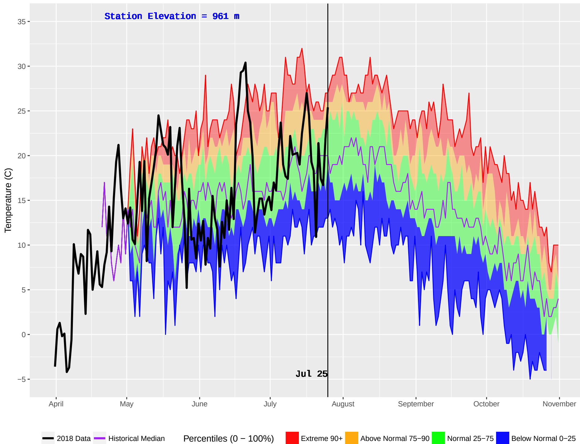
HOLY CROSS 2 (654) : Historical (1998–2016) and Current (2018) Noon Temperature
