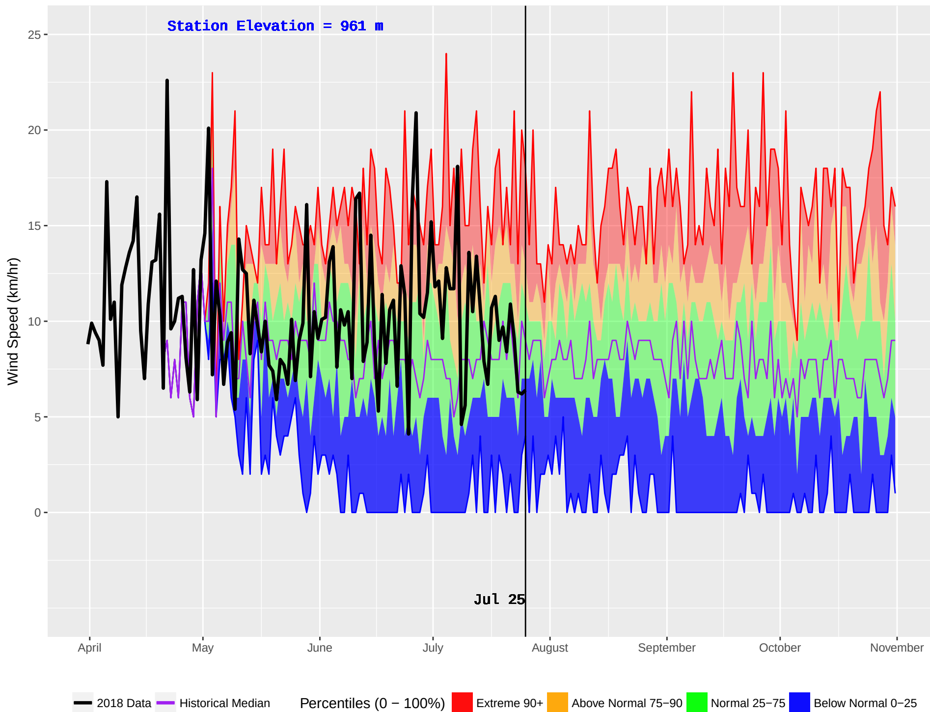
HOLY CROSS 2 (654) : Historical (1998–2016) and Current (2018) Noon Wind Speed
