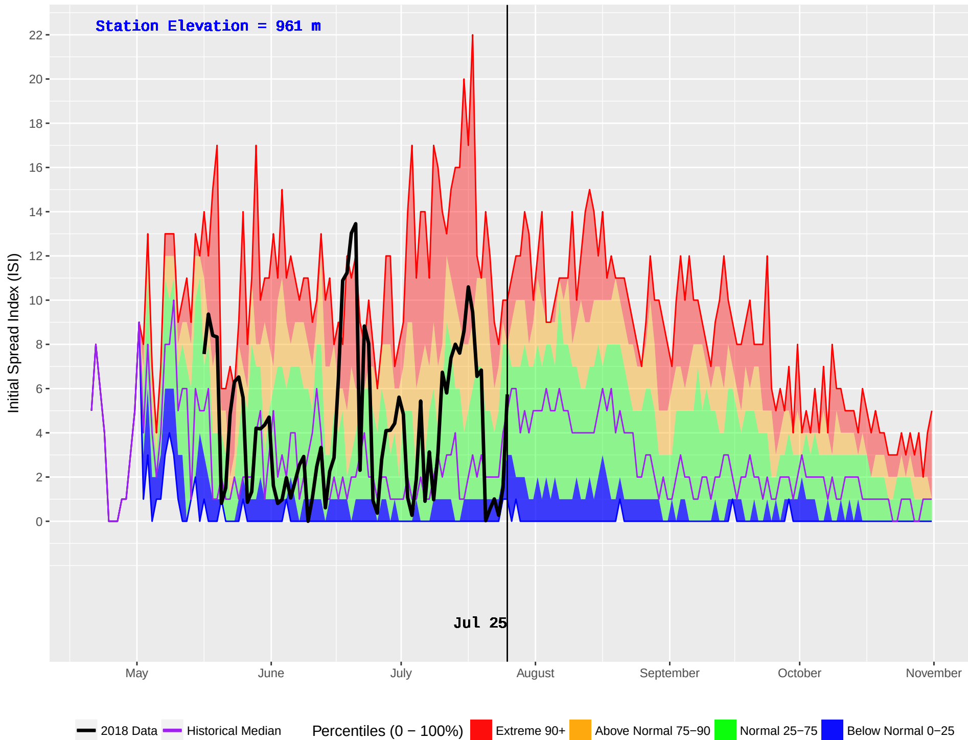
HOLY CROSS 2 (654) : Historical (1998–2016) and Current (2018) Noon Initial Spread Index (ISI)
