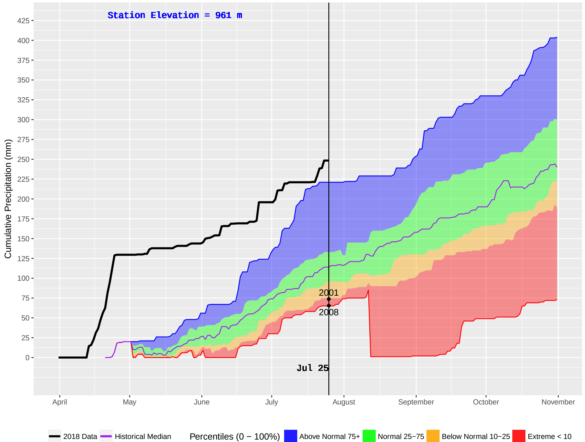
HOLY CROSS 2 (654) : Historical (1998–2016) and Current (2018) Noon Cumulative Precipitation
