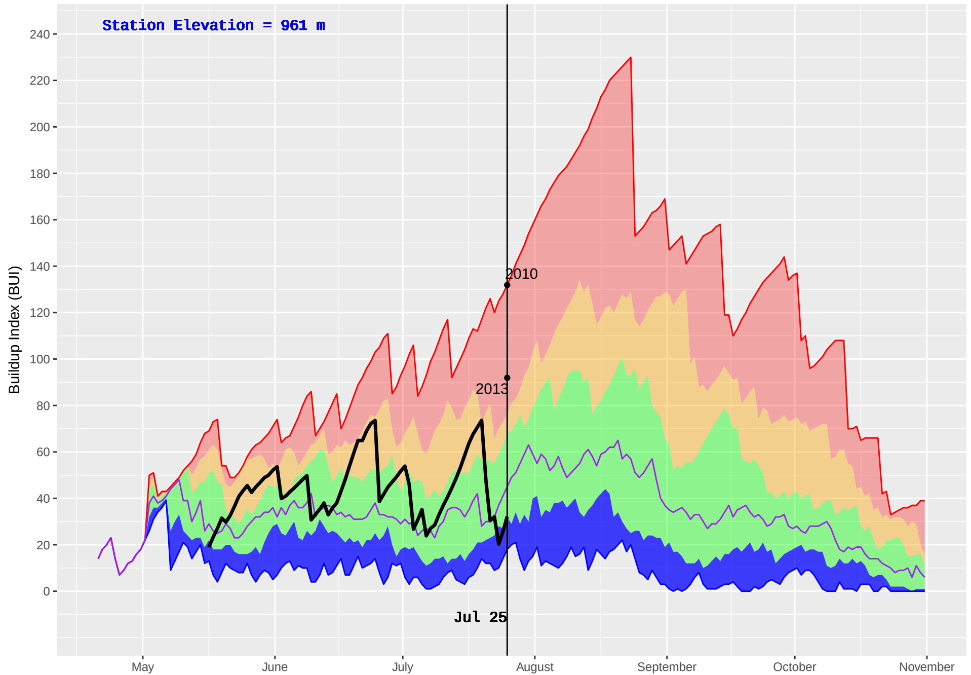
HOLY CROSS 2 (654) : Historical (1998–2016) and Current (2018) Noon Buildup Index (BUI)
