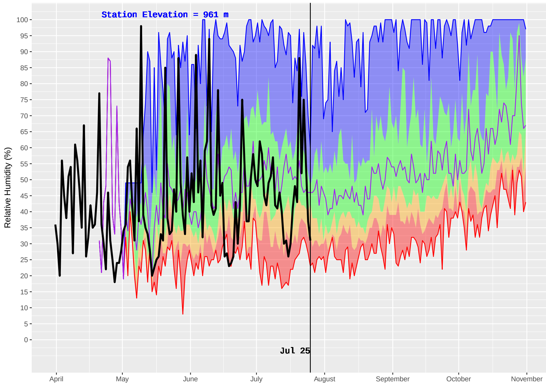
HOLY CROSS 2 (654) : Historical (1998–2016) and Current (2018) Noon Relative Humidity
