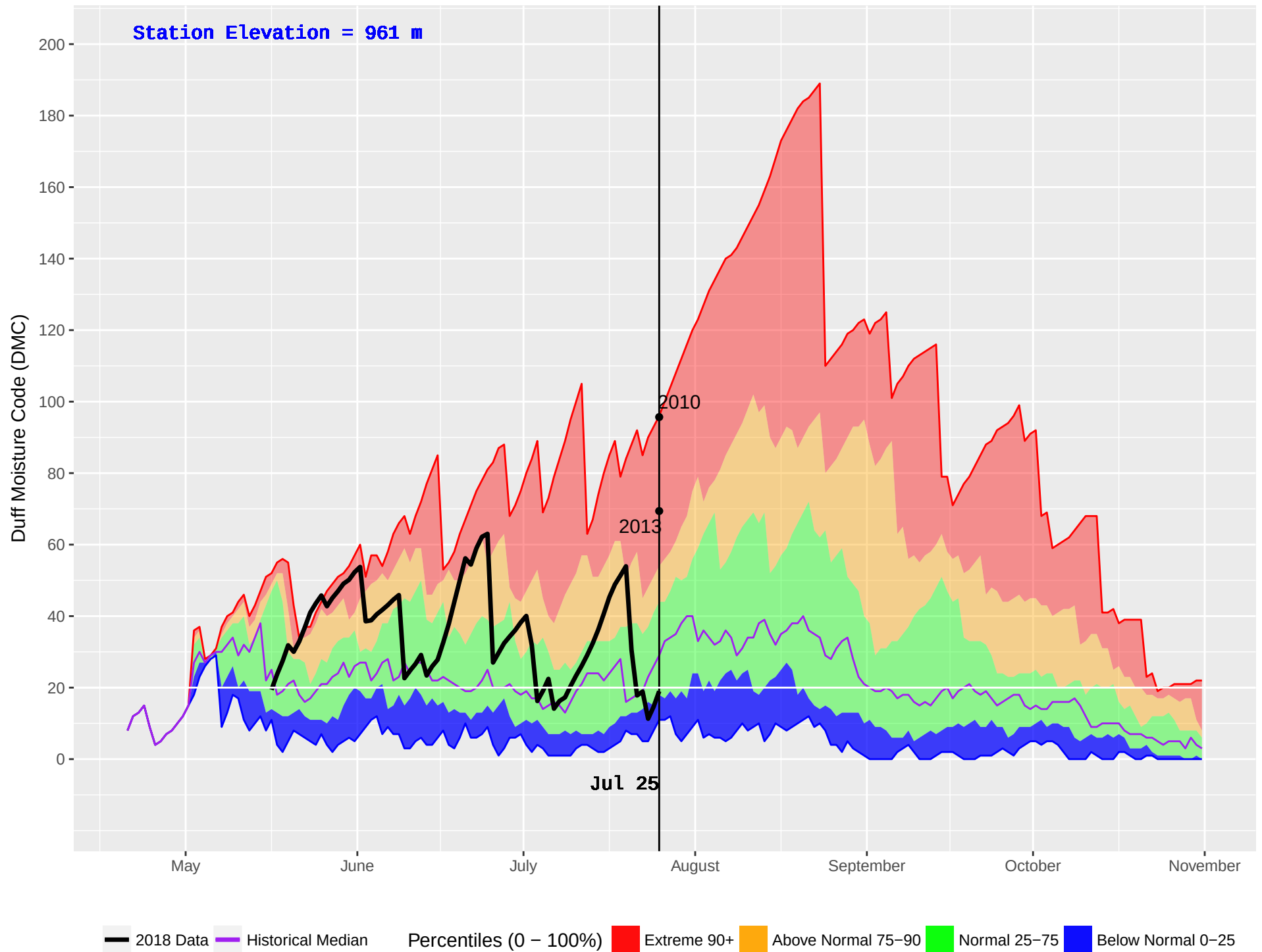
HOLY CROSS 2 (654) : Historical (1998–2016) and Current (2018) Noon Duff Moisture Code (DMC)
