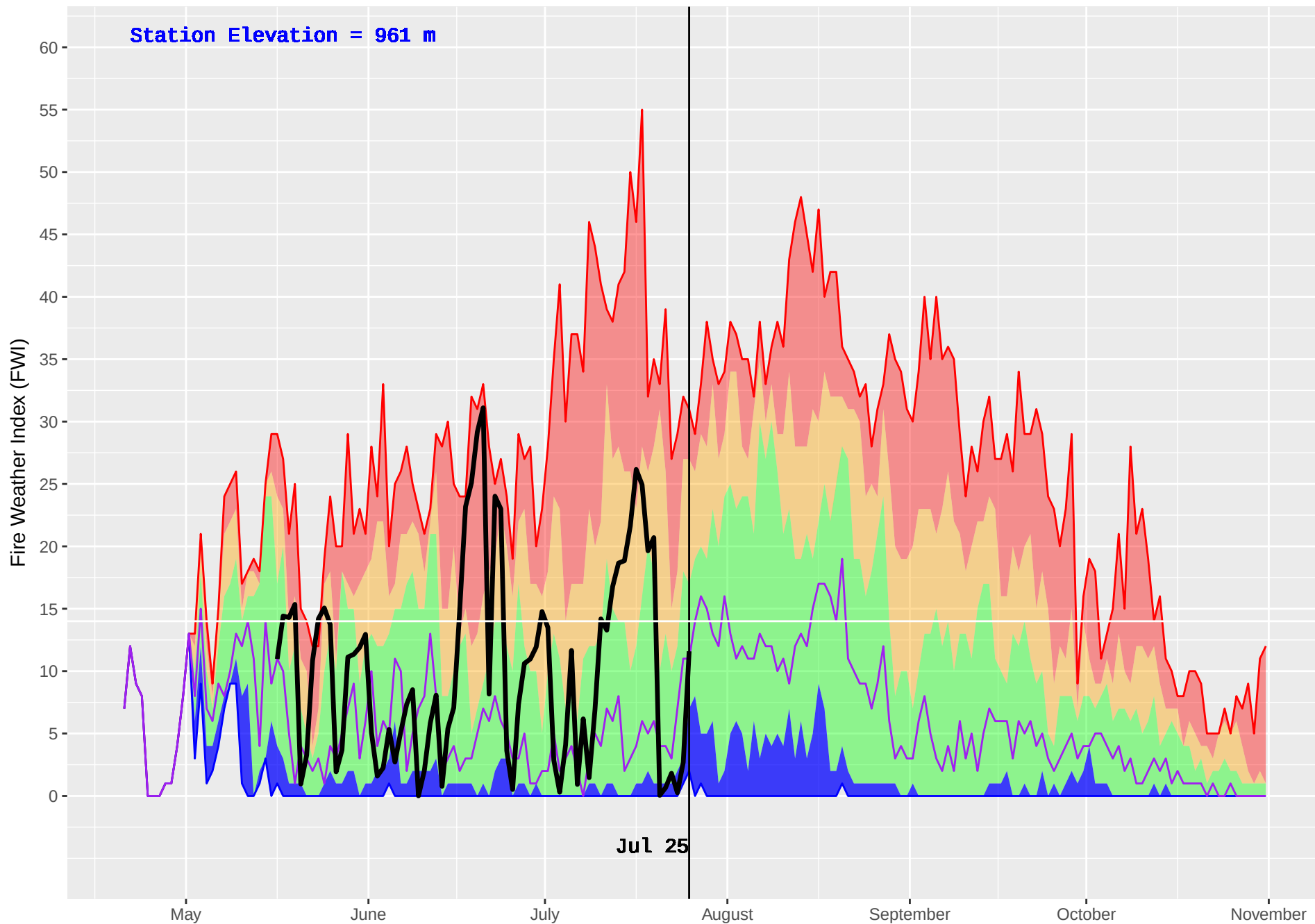
HOLY CROSS 2 (654) : Historical (1998–2016) and Current (2018) Noon Fire Weather Index (FWI)
